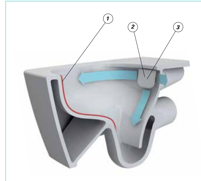
Standard WC pan
